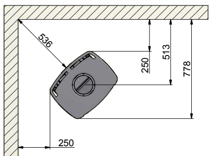
65-2, 65-4, 65-8 and 65-10 (with side windows) 45° corner installation
