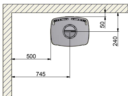
65-2, 65-4, 65-8 and 65-10 (with side windows) Parallel installation
