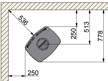
41-2 (with side windows) 45° corner installation
