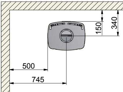
41-2 (with side windows) Parallel installation
