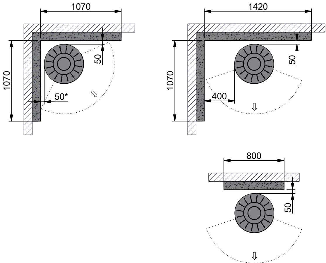
Minimum distance to flammable wall protected by a fire wall
