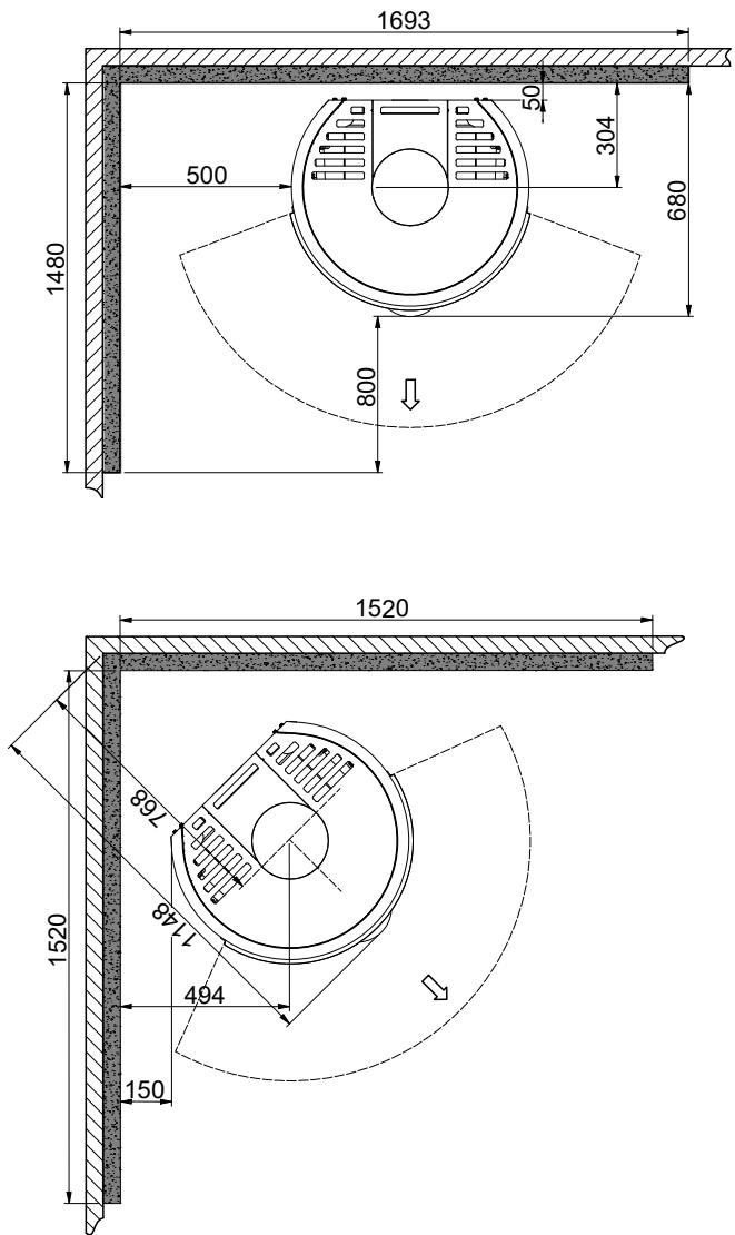
Minimum distance to flammable wall protected by a fire wall
