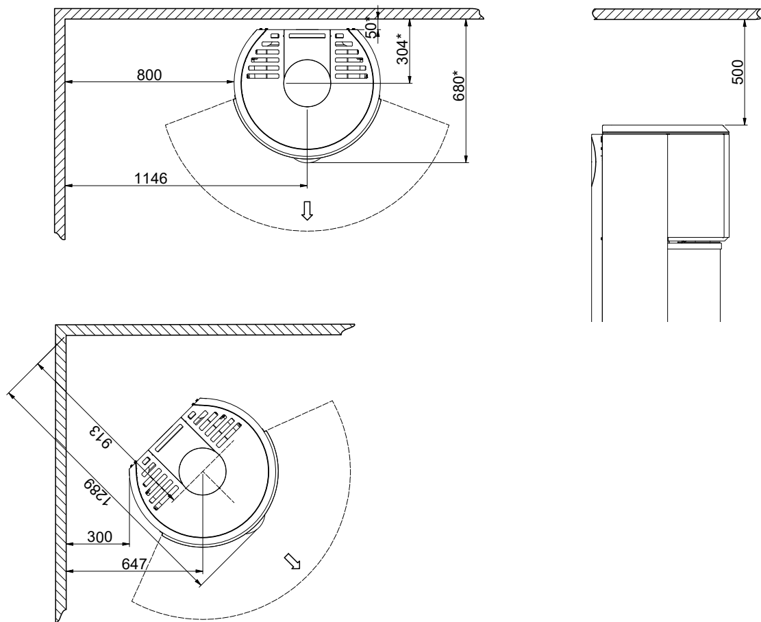
Minimum distance to flammable materials
